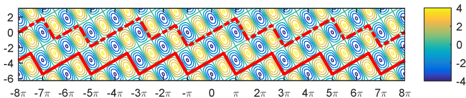
FIG. 2. Contour of the total field u given by (3.2). The red solid line and the red dash-dot line denote two grating curves with different minimum periods, respectively.
