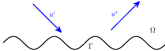
FIG. 1. Scattering by a periodic curve with Dirichlet boundary condition.
