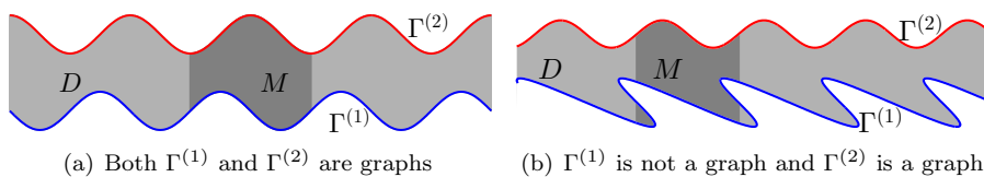
FIG. 4. The unbounded periodic strip D and its one periodicity cell M in Case (ii): \Gamma^{(1)} \cap \Gamma^{(2)} = \emptyset .
